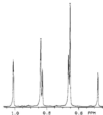
Figure 1. 360-MHz 1 H NMR spectrum of C(11)H 3 and C(12)H 3 in the product mixture 11 and 12 + 13 from chloro olefin 10 . The upfield methyl is C(11); the dominant labeled methyl is 13 C(12).
