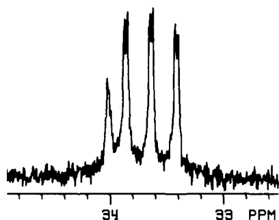
Figure 4. The C(10) region of the proton-decoupled ^{13}\text{C} NMR spectrum of the product from chloro olefin 10 ; J_{^{13}\text{C}-\text{D}} = 20 Hz, J_{^{13}\text{C}-\text{C}-^{13}\text{C}(11,12)} = 2 Hz.
