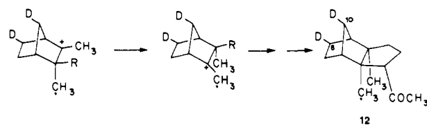
Scheme II. Minor Stereochemical Path without Endo Shift a
