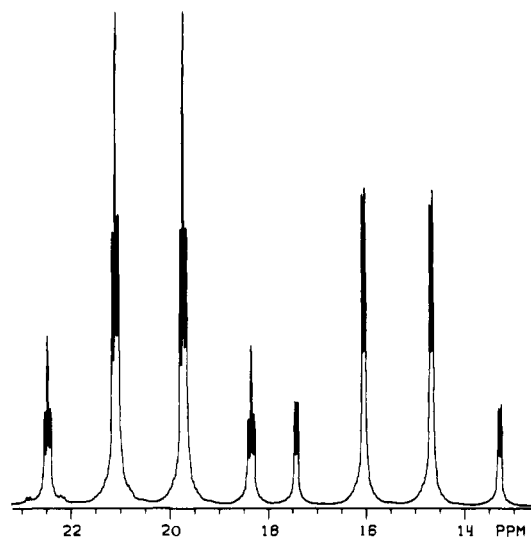
Figure 2. Long-range ^{13}\text{C} -C-C-H spin-spin coupling at C(12) (downfield methyl) and C(11) in the product mixture 11 and 12 + 13 from chloro olefin 10 .
