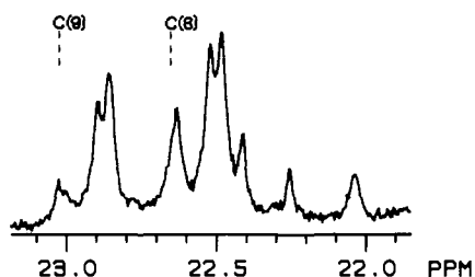
Figure 5. Observed natural abundance C(8) and C(9) proton-decoupled ^{13}\text{C} NMR spectrum for ketones 11 + 12 from the chloro annelation of 10 .
