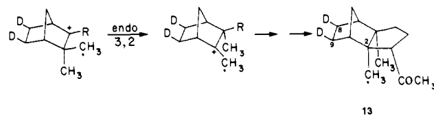
Scheme III. Minor Stereochemical Path with Endo Shift a
