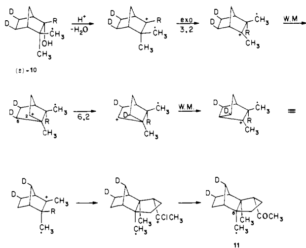
Scheme I. Major Stereochemical Path a
